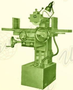
UNIVERSAL HEAD FIXED
